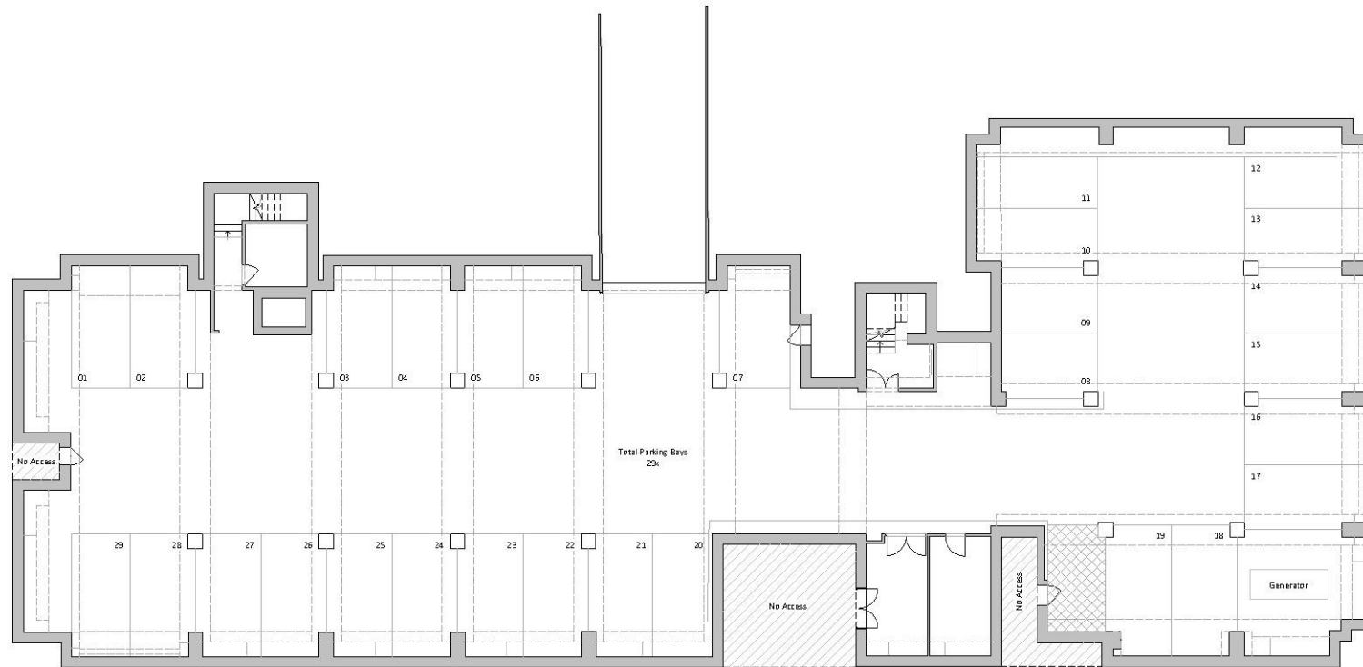
-01 Proposed Basement Floor NB.1 1:100
